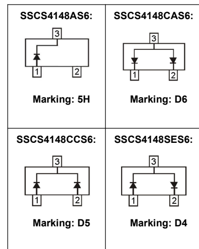
Circuit Diagram
